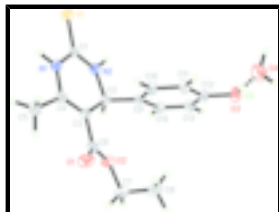
Fig. 1. The molecular structure of the title molecule, with the atom-numbering scheme. Displacement ellipsoids are drawn at the 50% probability level. Hydrogen bond is shown as dashed lines.
